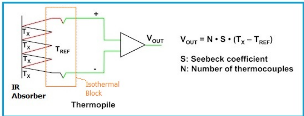
Thermopile Structure and Mathematical Equation (Reference: rfwireless-world.com )
