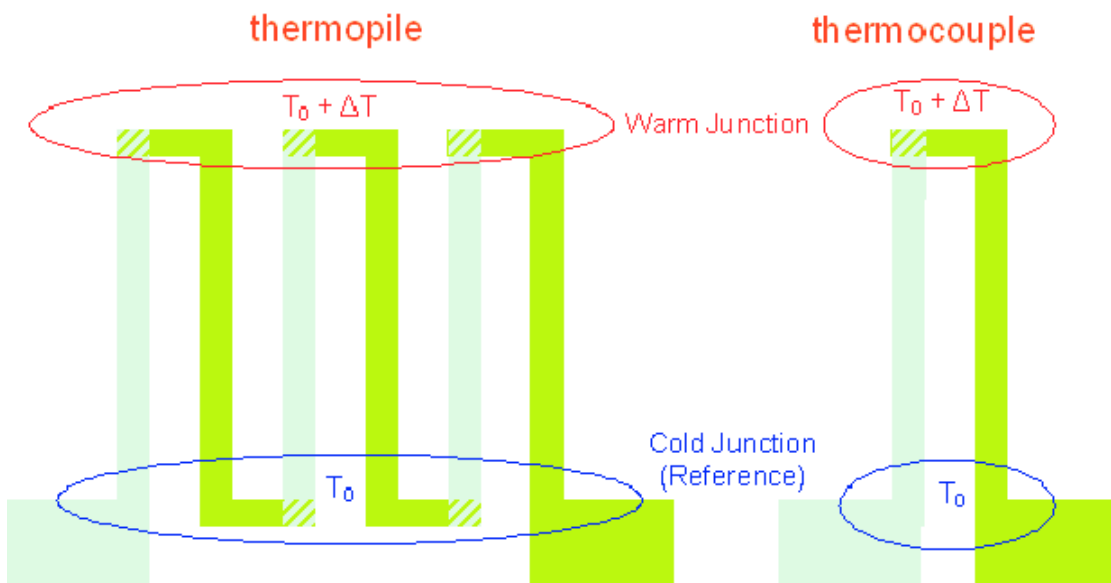
A schematic diagram of thermocouple and thermopile (Reference: researchgate.net )
